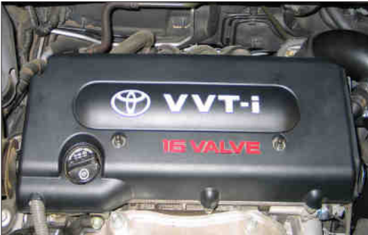
33. Install the stock engine cover and secure with the stock mounting bolts removed in step #10.
